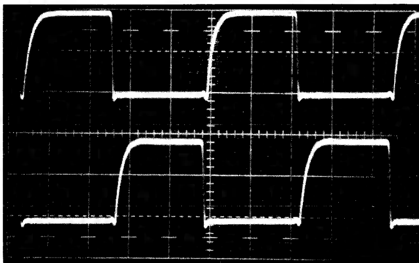
FIGURE 3.6b – Proper Clocks
